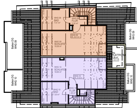
WHG 10 27.23 m 2
