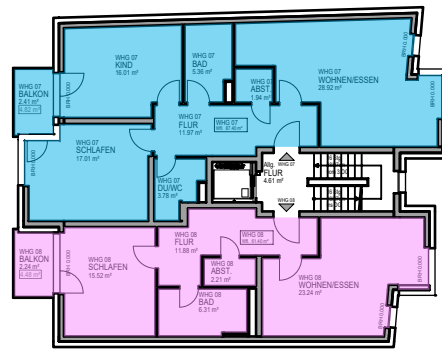
WHG 08 61.40 m 2
